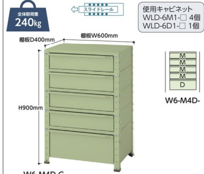
W6-M4D-G W6-M4D- 質量:54.5kg ¥134,330
